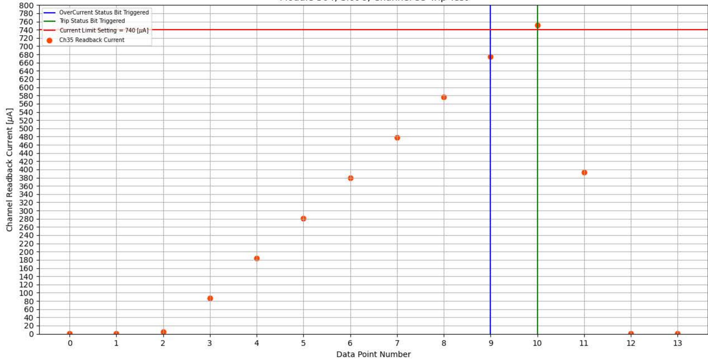
Module 304, Slot 8, Channel 35 Trip Test
