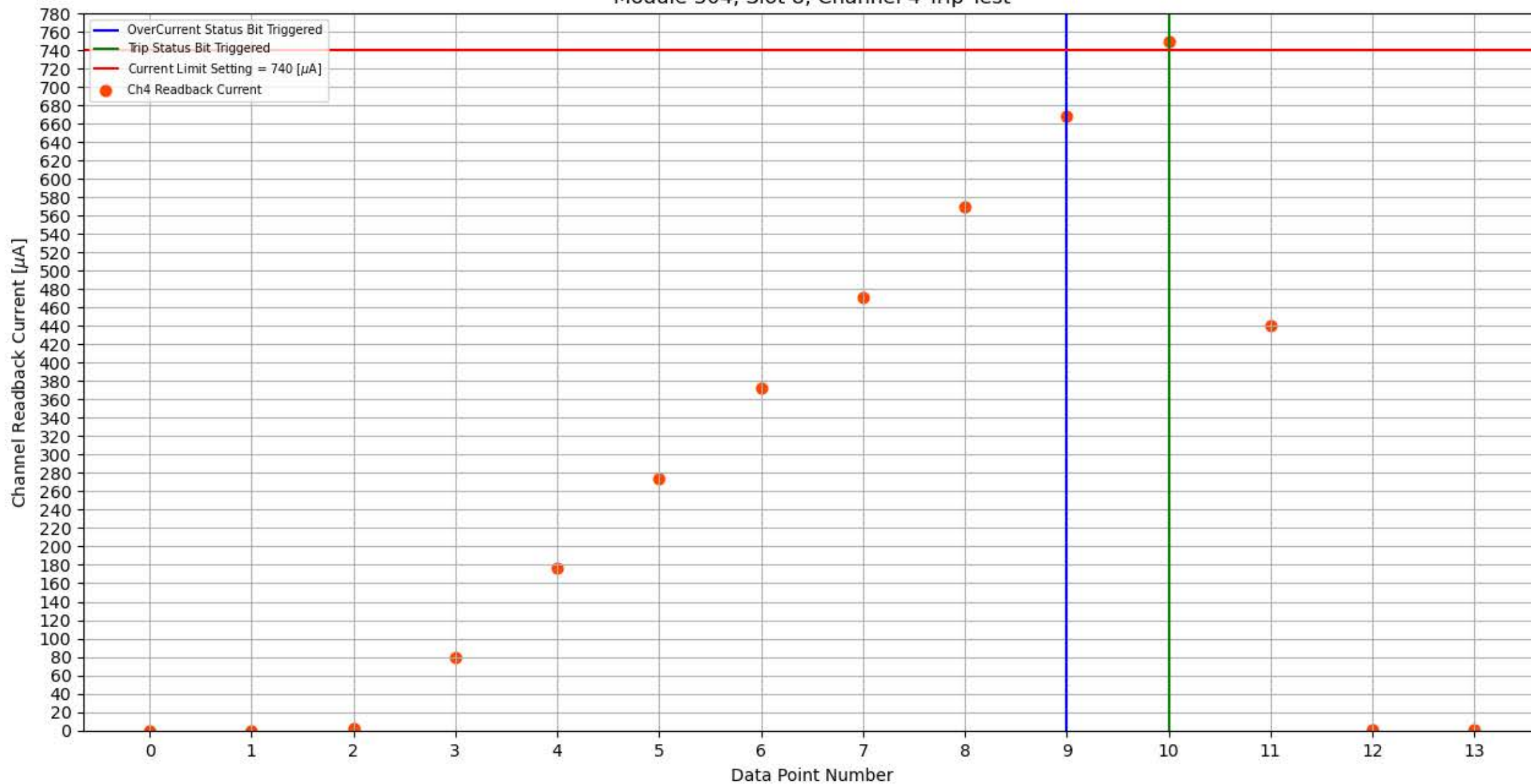
Module 304, Slot 8, Channel 4 Trip Test
