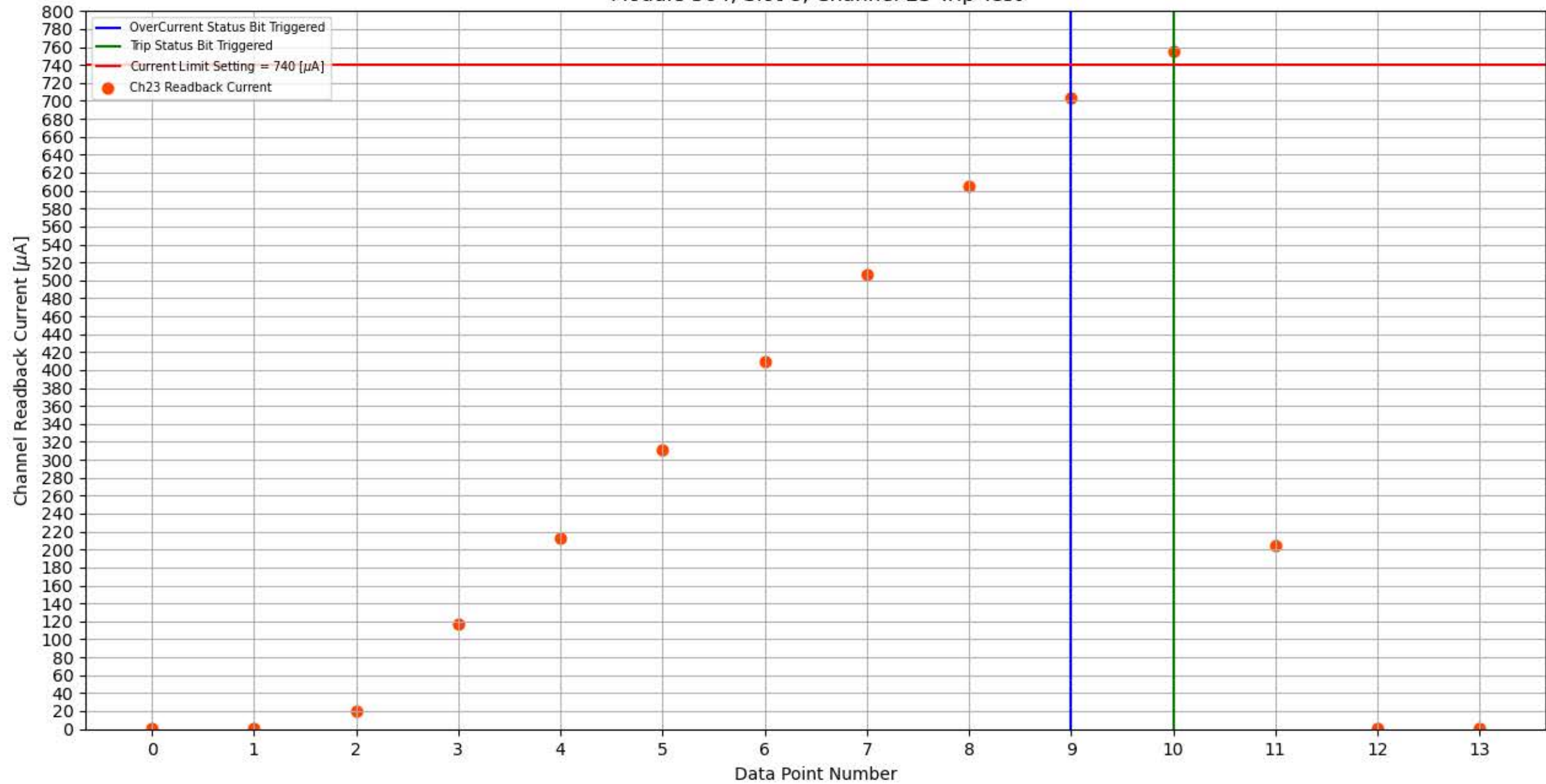
Module 304, Slot 8, Channel 23 Trip Test
