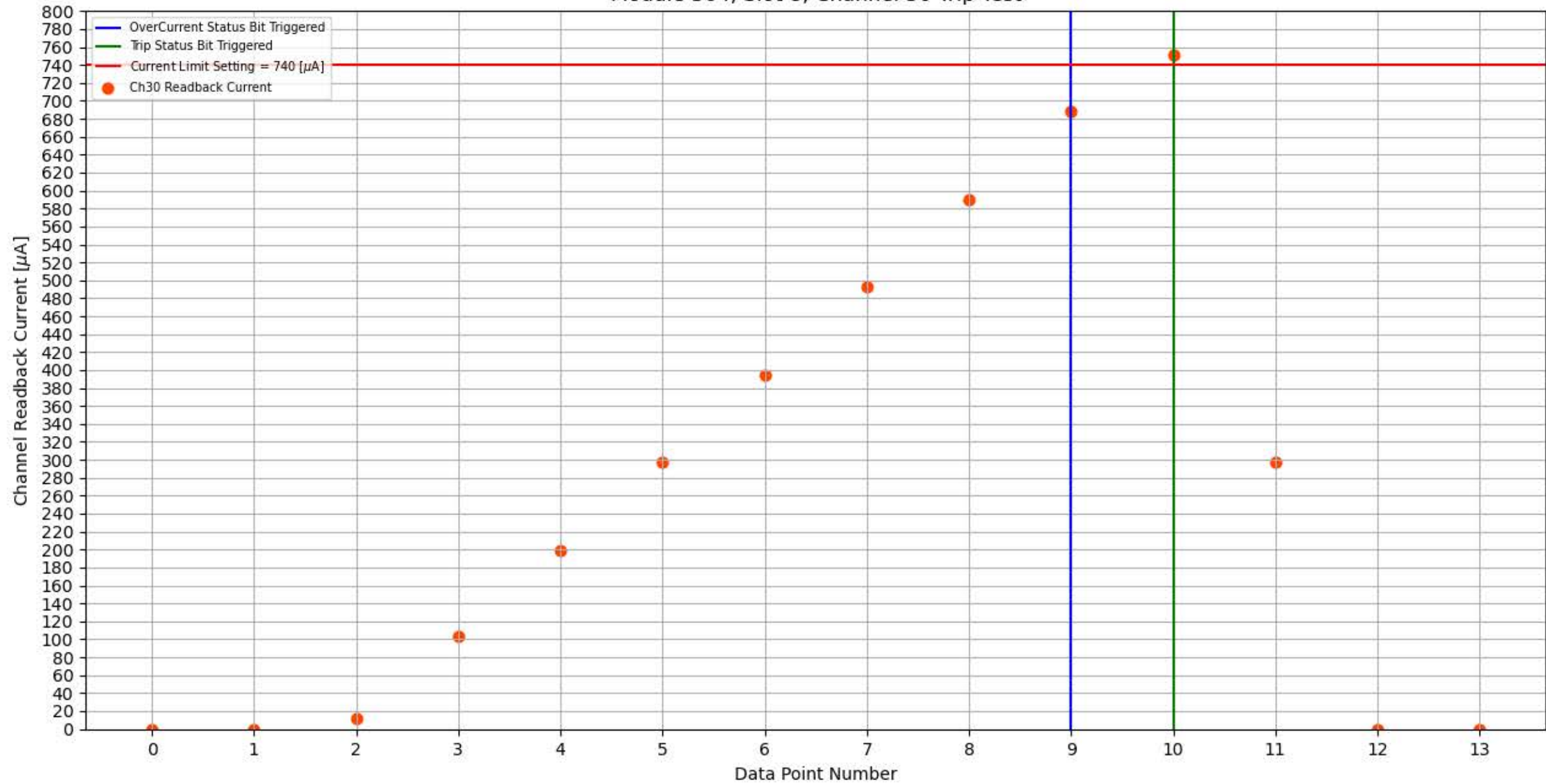
Module 304, Slot 8, Channel 30 Trip Test
