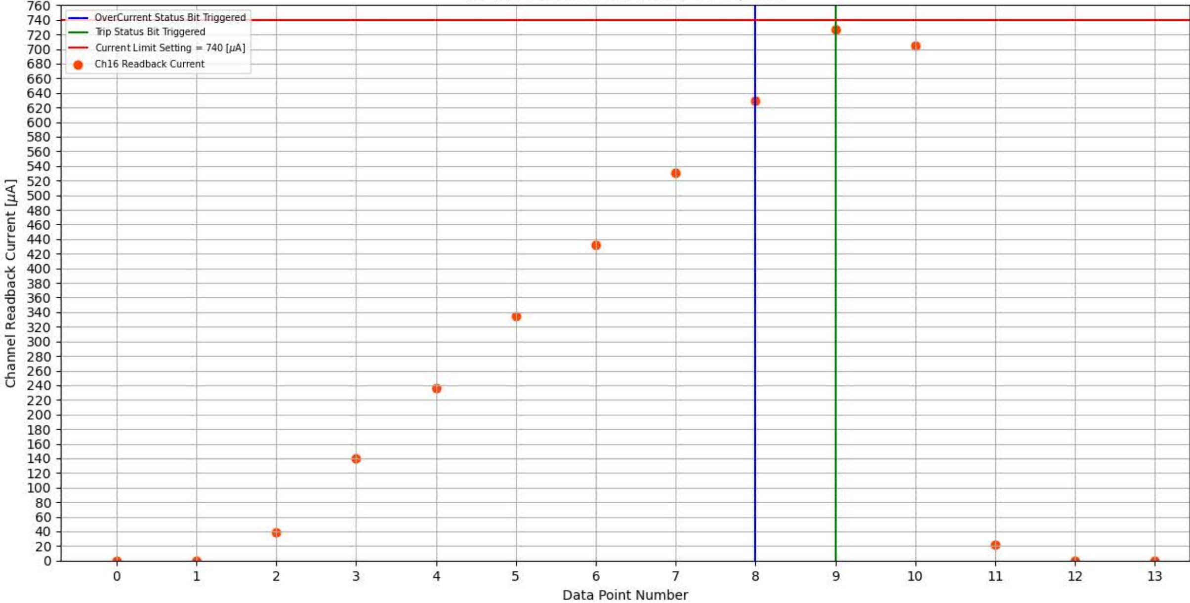
Module 304, Slot 8, Channel 16 Trip Test
