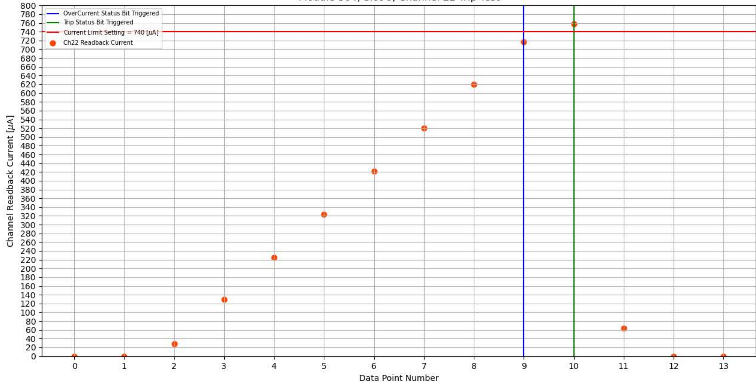
Module 304, Slot 8, Channel 22 Trip Test
