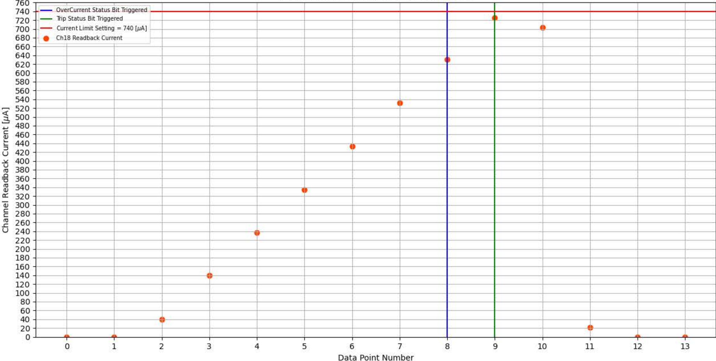
Module 304, Slot 8, Channel 18 Trip Test
