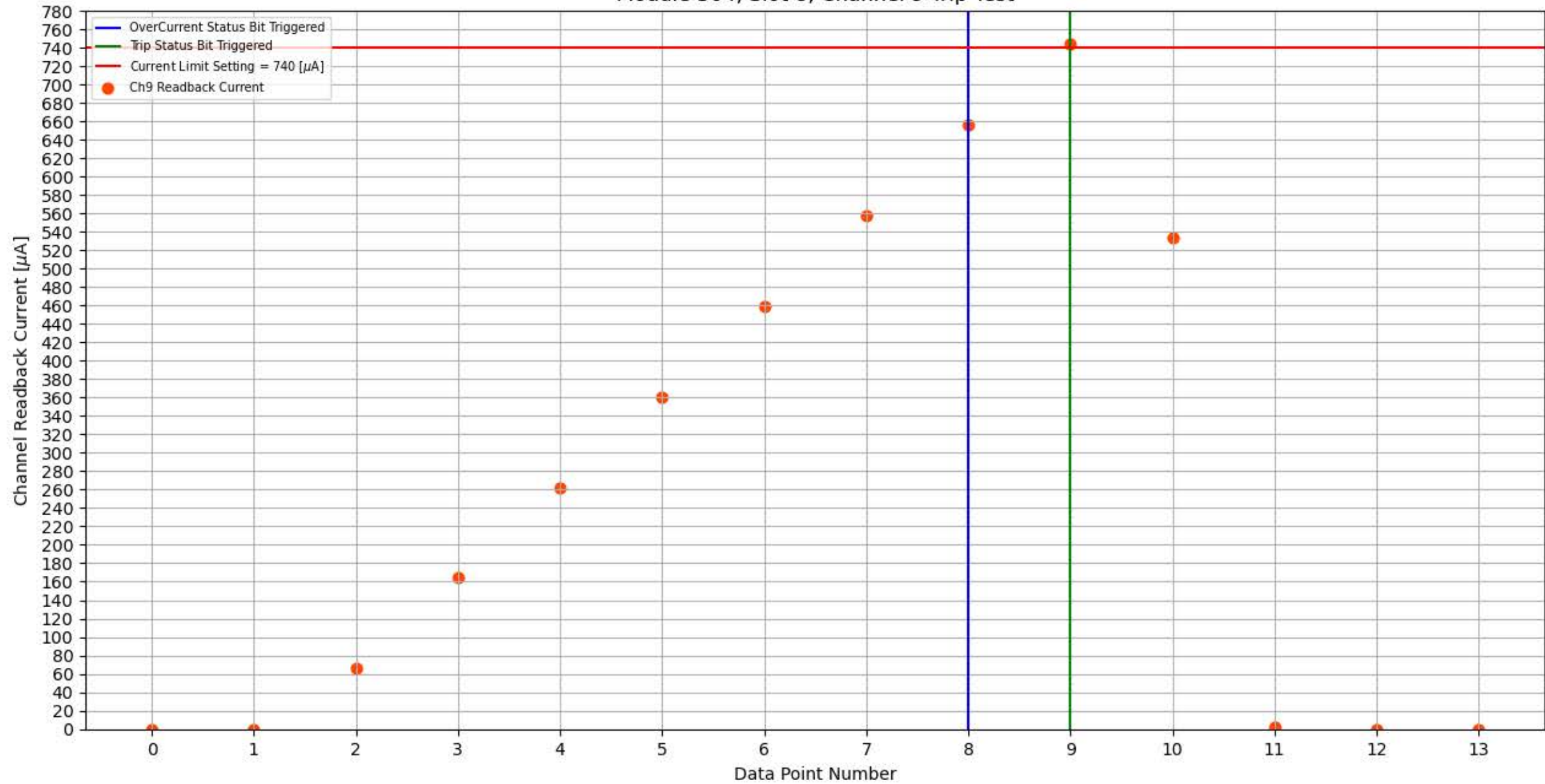
Module 304, Slot 8, Channel 9 Trip Test
