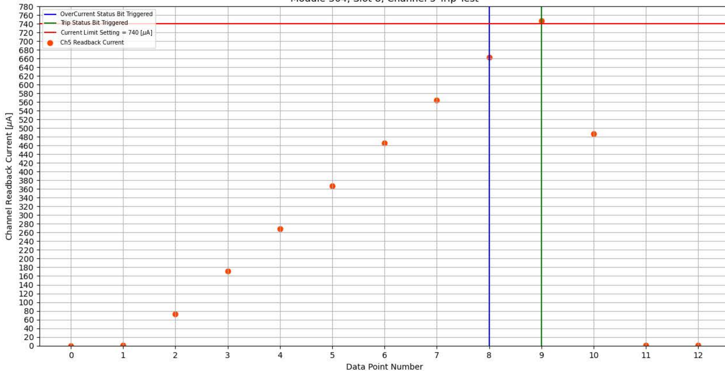
Module 304, Slot 8, Channel 5 Trip Test
