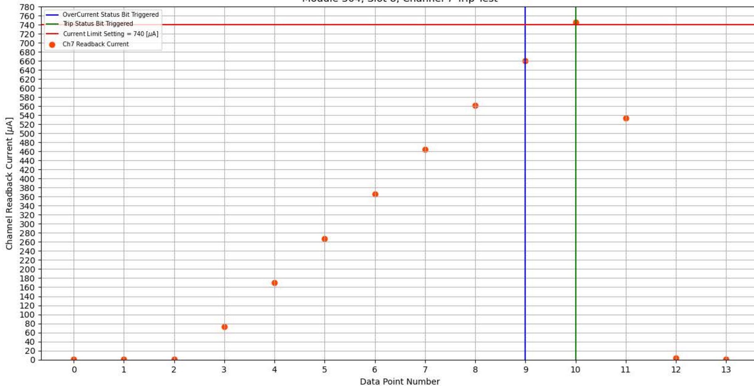
Module 304, Slot 8, Channel 7 Trip Test
