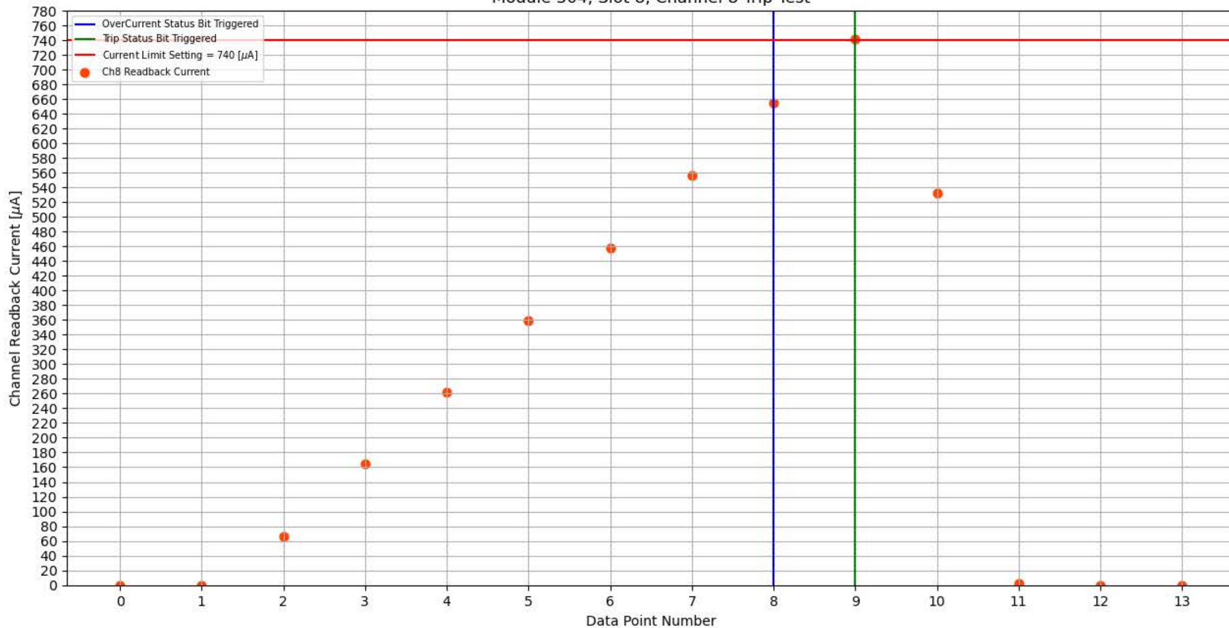
Module 304, Slot 8, Channel 8 Trip Test
