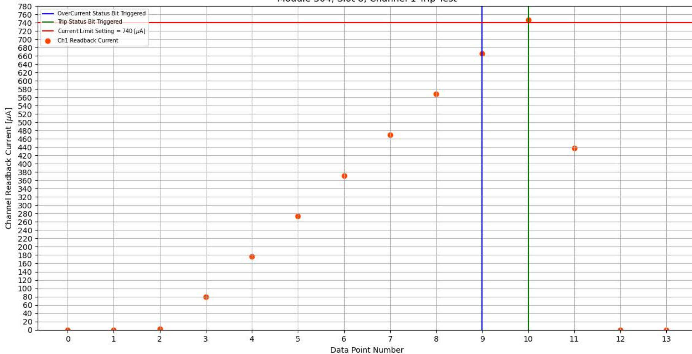
Module 304, Slot 8, Channel 1 Trip Test
