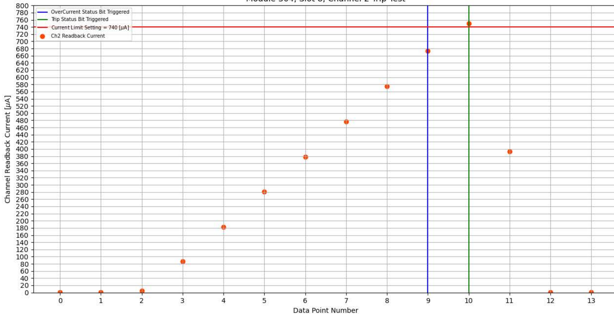
Module 304, Slot 8, Channel 2 Trip Test
