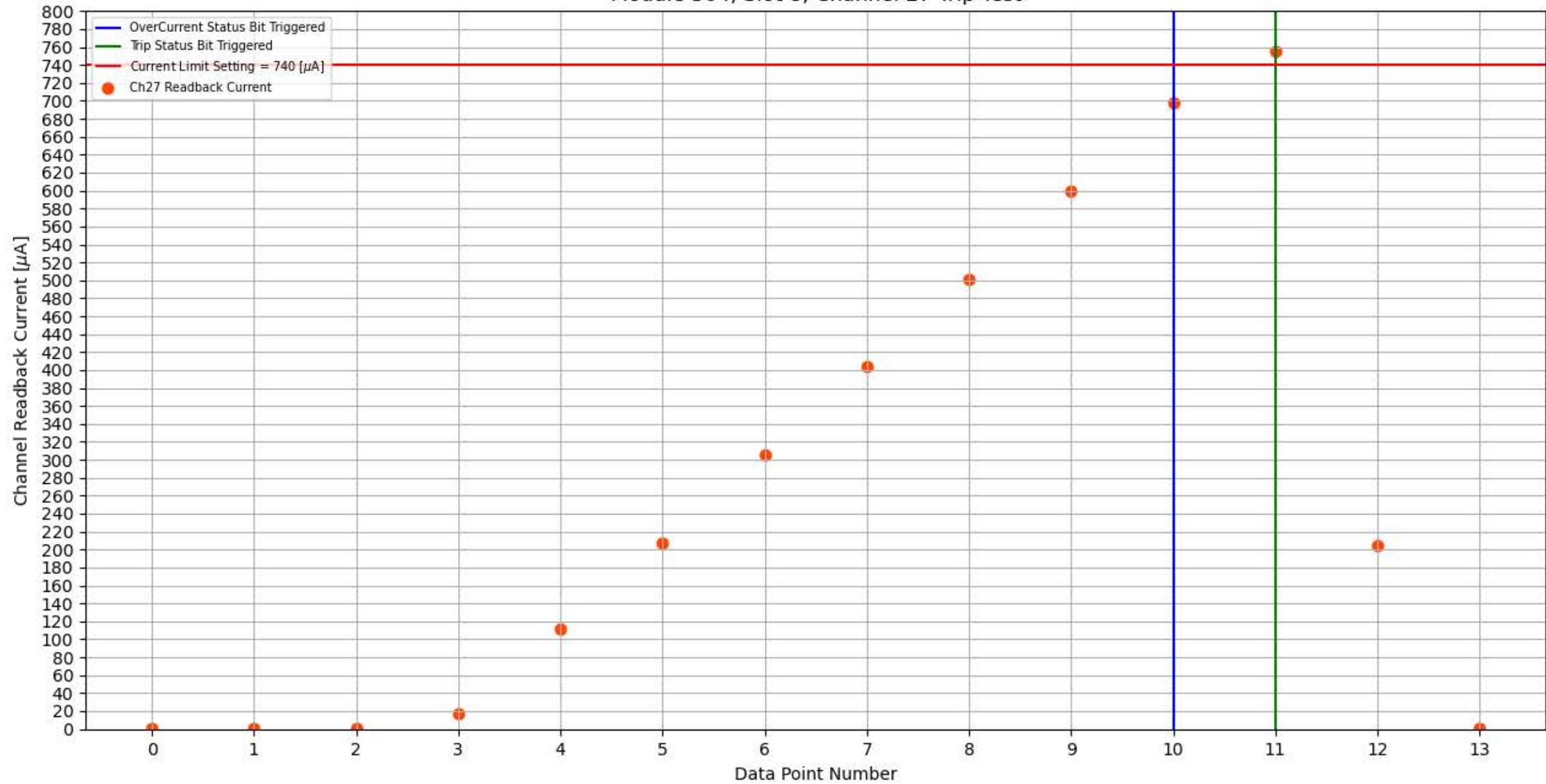
Module 304, Slot 8, Channel 27 Trip Test
