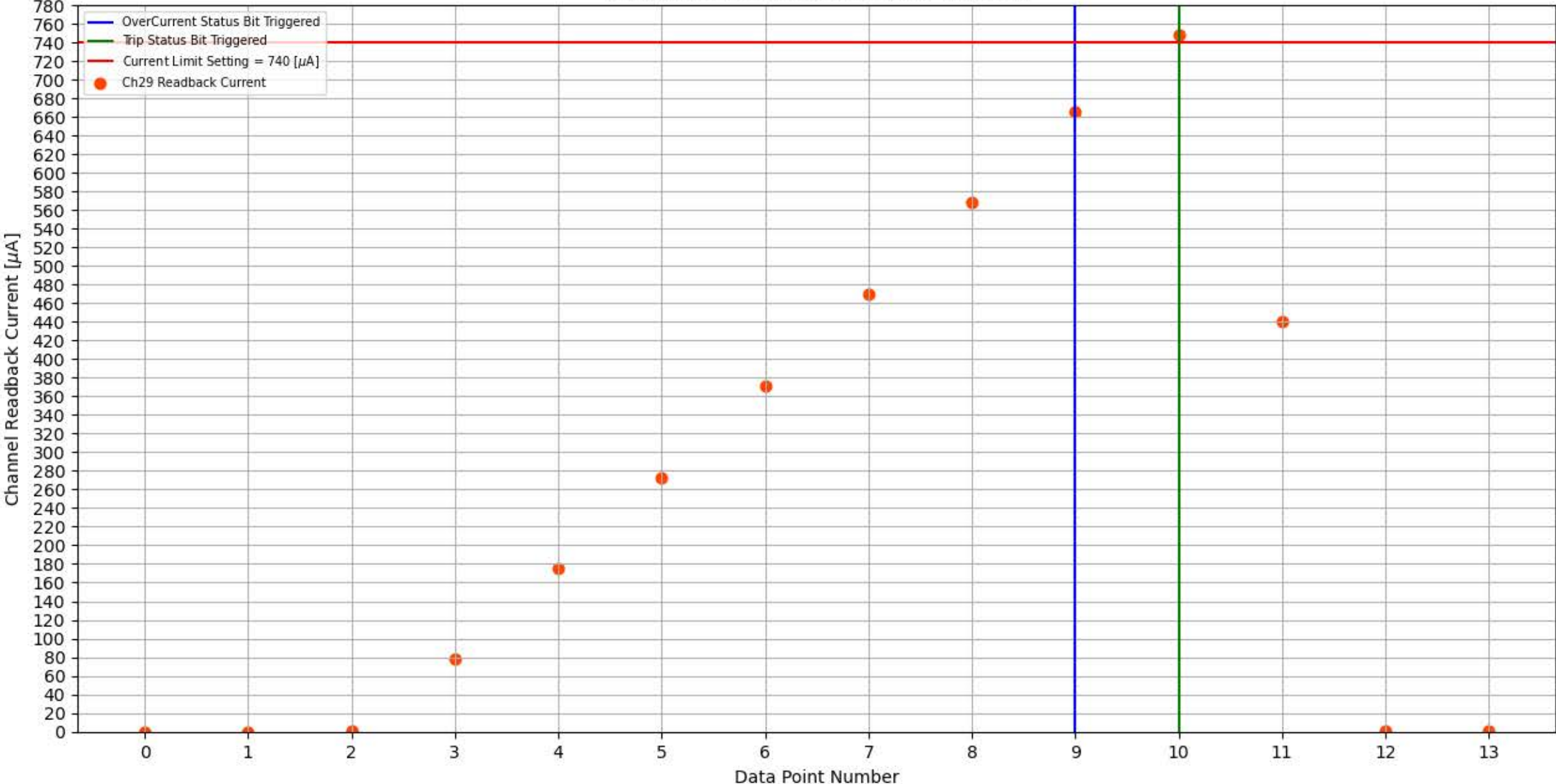
Module 304, Slot 8, Channel 29 Trip Test
