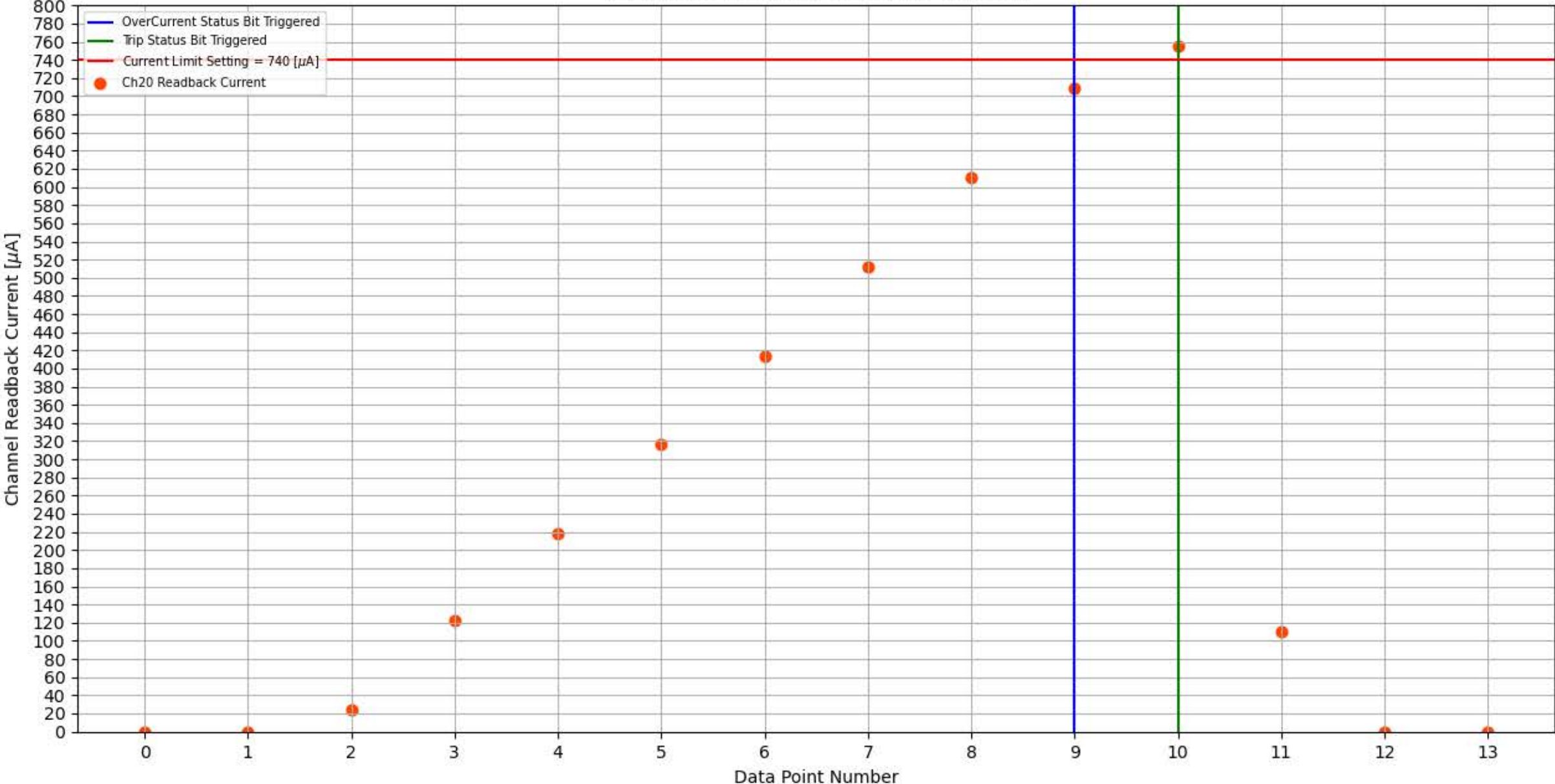
Module 304, Slot 8, Channel 20 Trip Test
