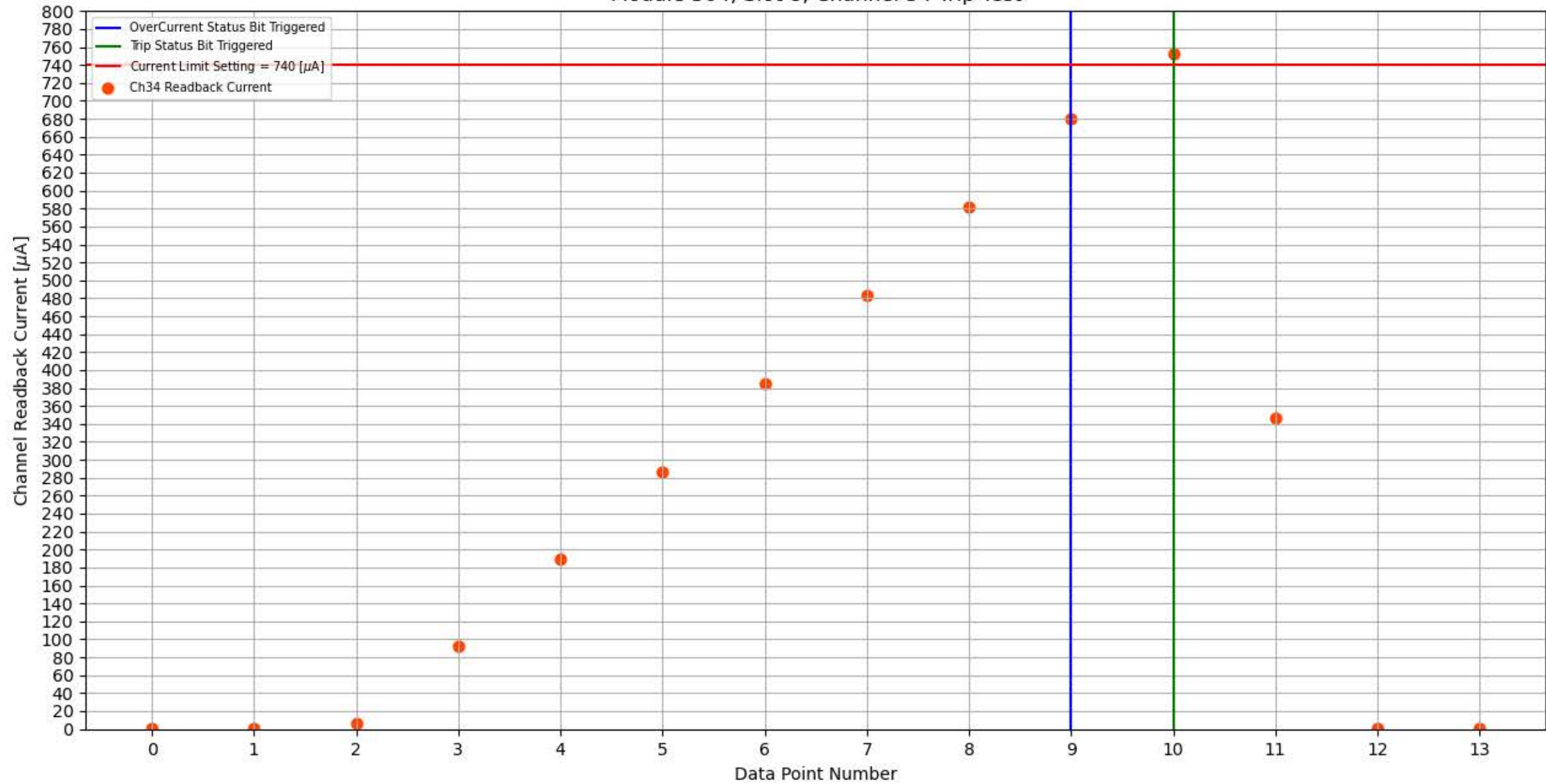
Module 304, Slot 8, Channel 34 Trip Test
