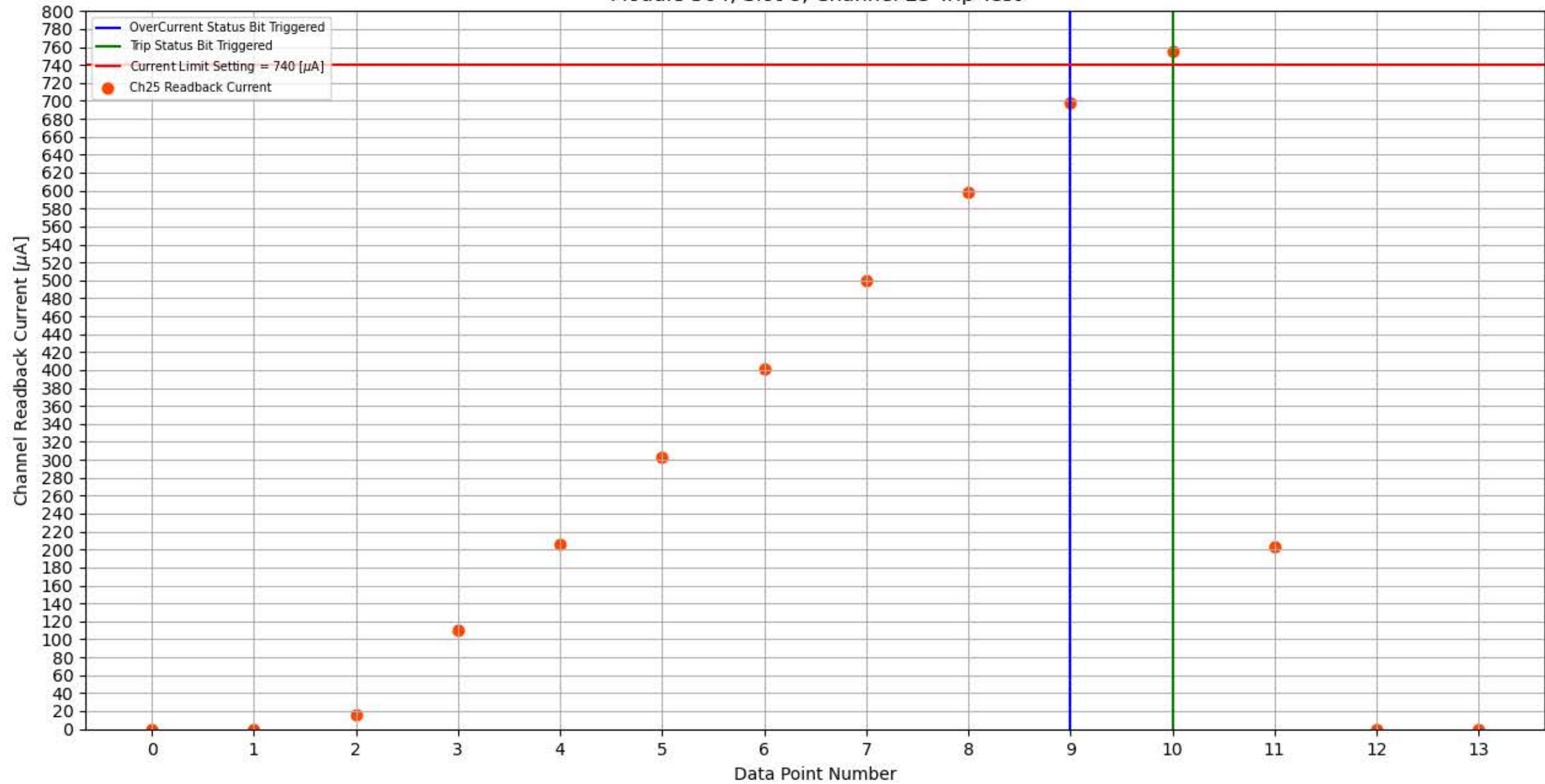
Module 304, Slot 8, Channel 25 Trip Test
