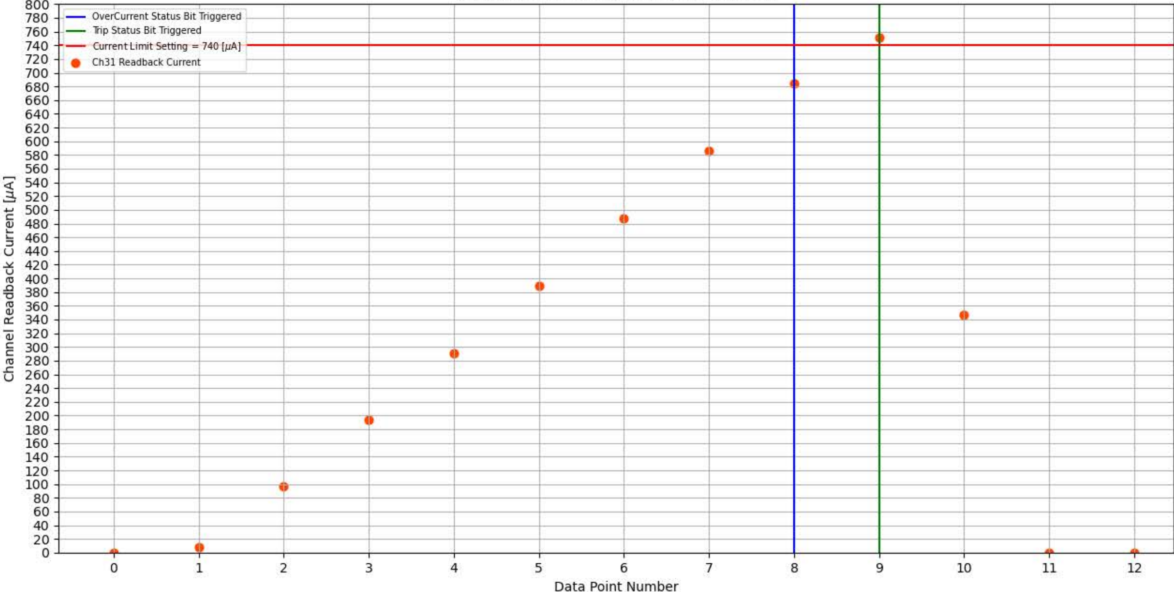
Module 304, Slot 8, Channel 31 Trip Test
