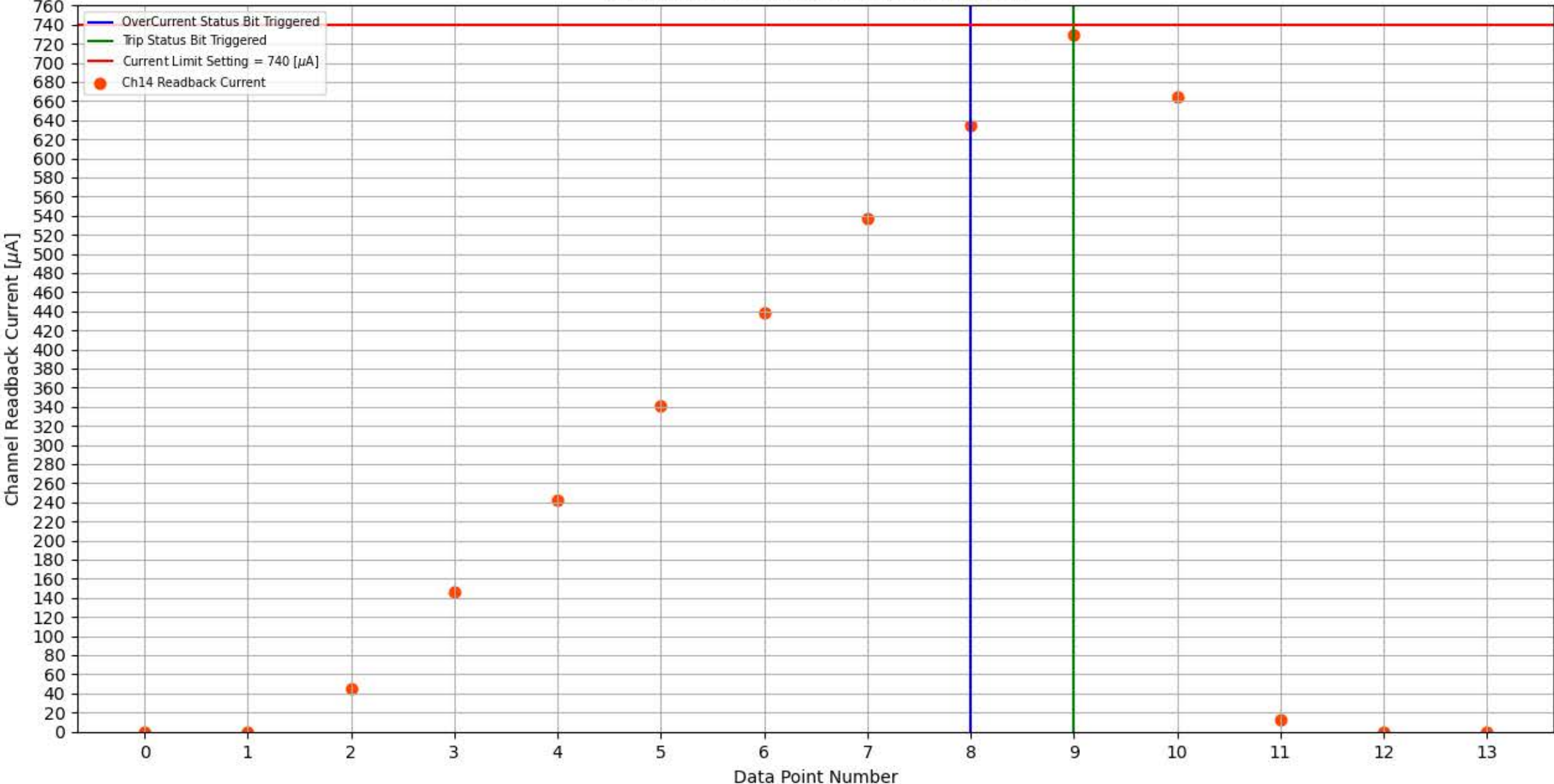
Module 304, Slot 8, Channel 14 Trip Test
