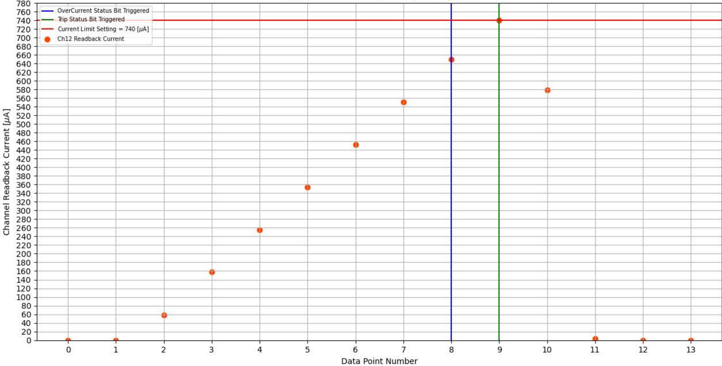
Module 304, Slot 8, Channel 12 Trip Test
