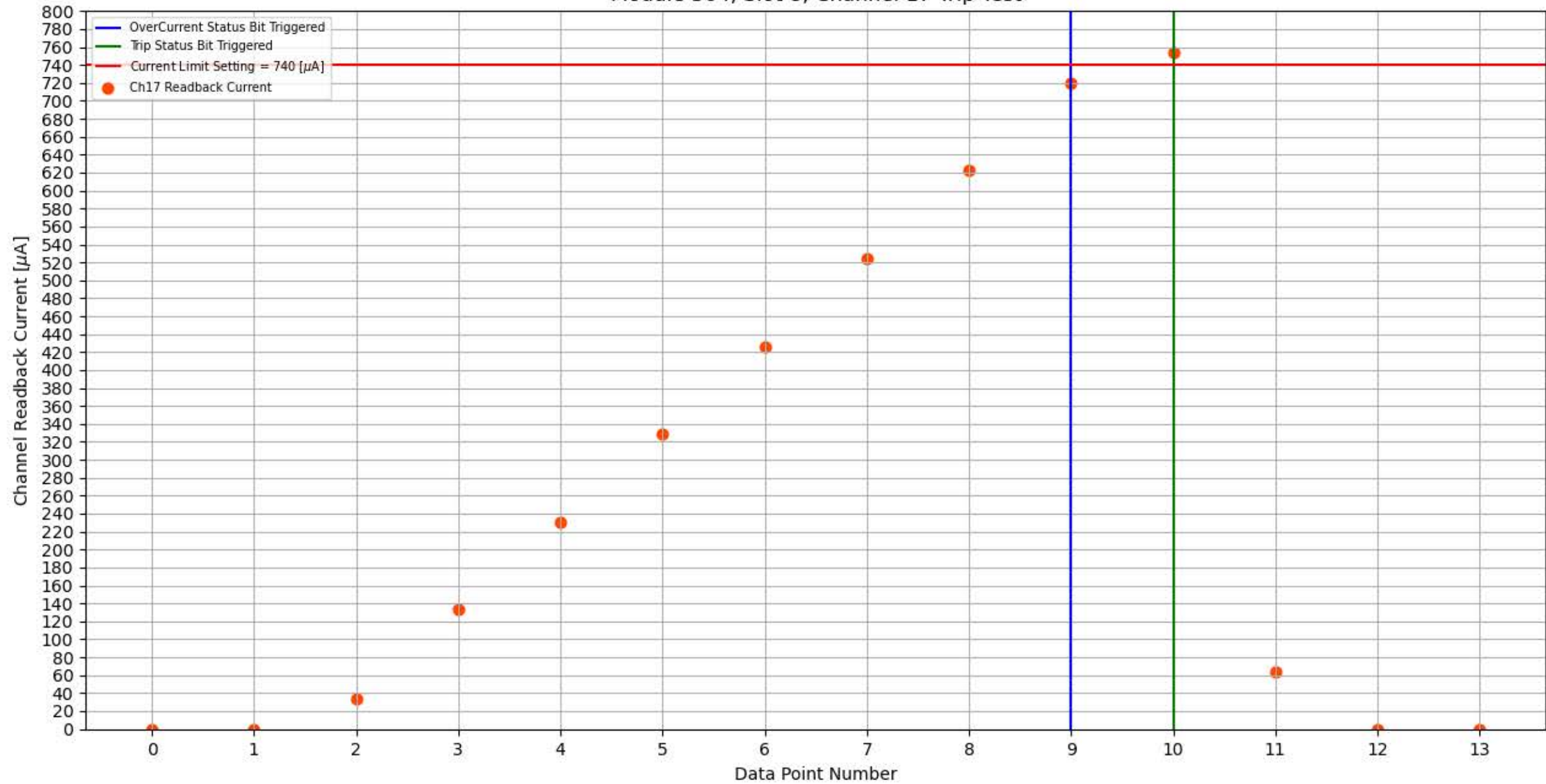
Module 304, Slot 8, Channel 17 Trip Test
