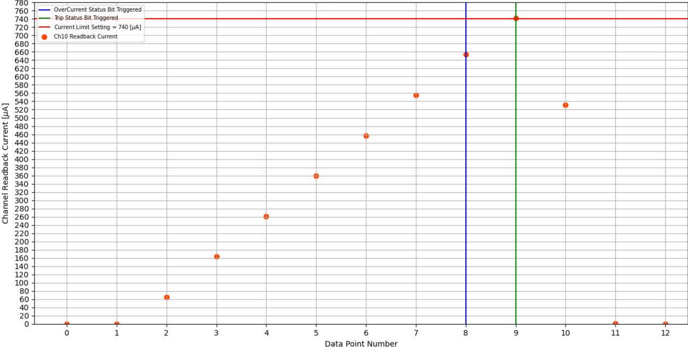
Module 304, Slot 8, Channel 10 Trip Test
