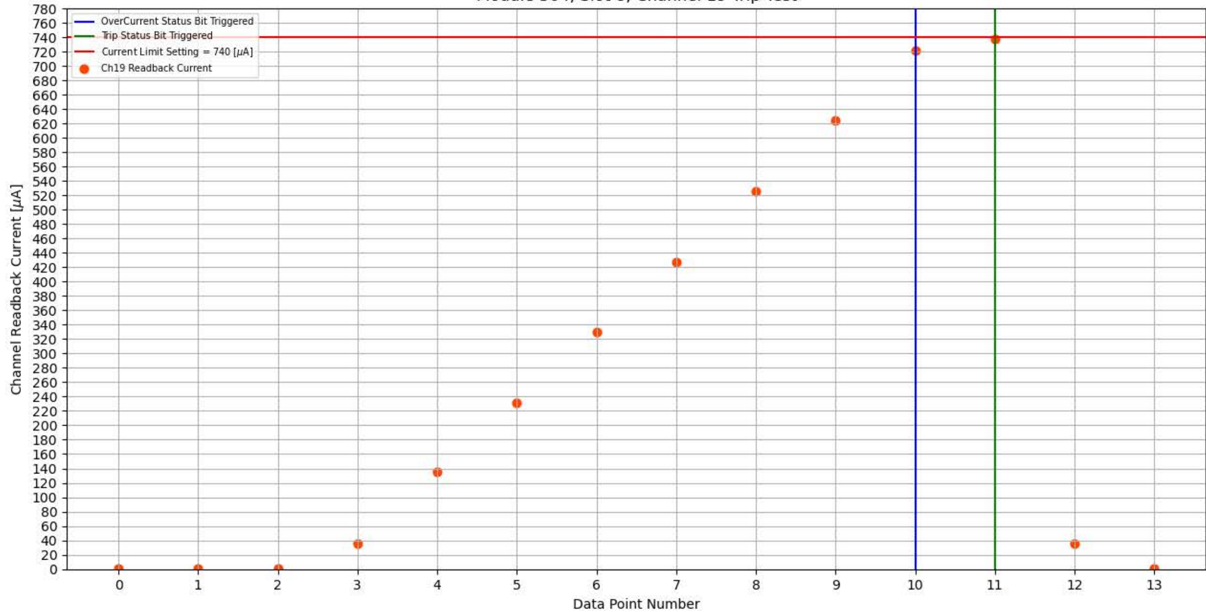
Module 304, Slot 8, Channel 19 Trip Test
