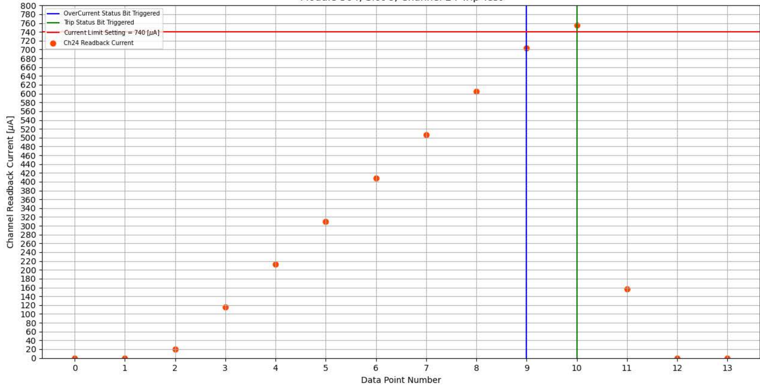
Module 304, Slot 8, Channel 24 Trip Test
