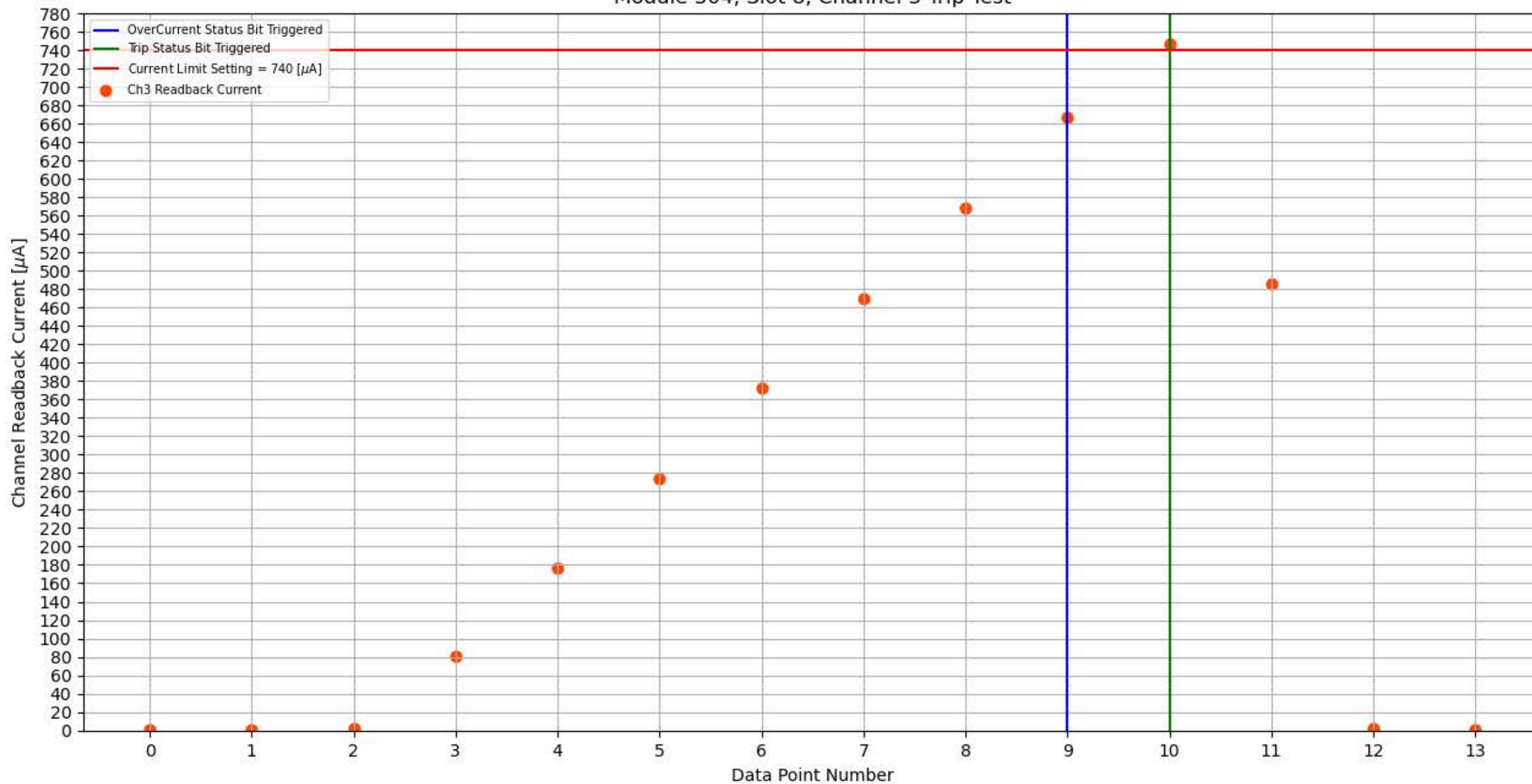
Module 304, Slot 8, Channel 3 Trip Test
