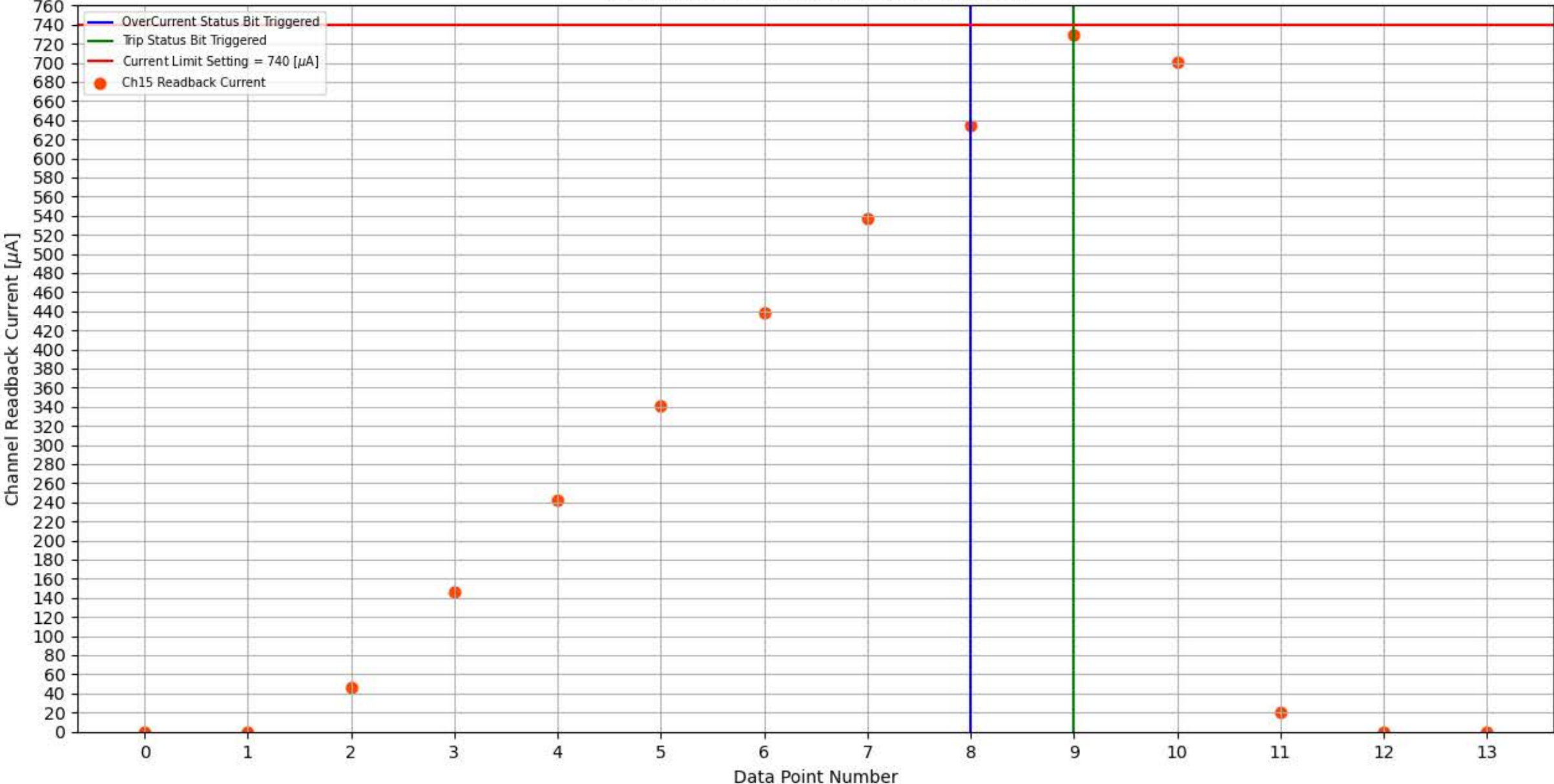
Module 304, Slot 8, Channel 15 Trip Test
