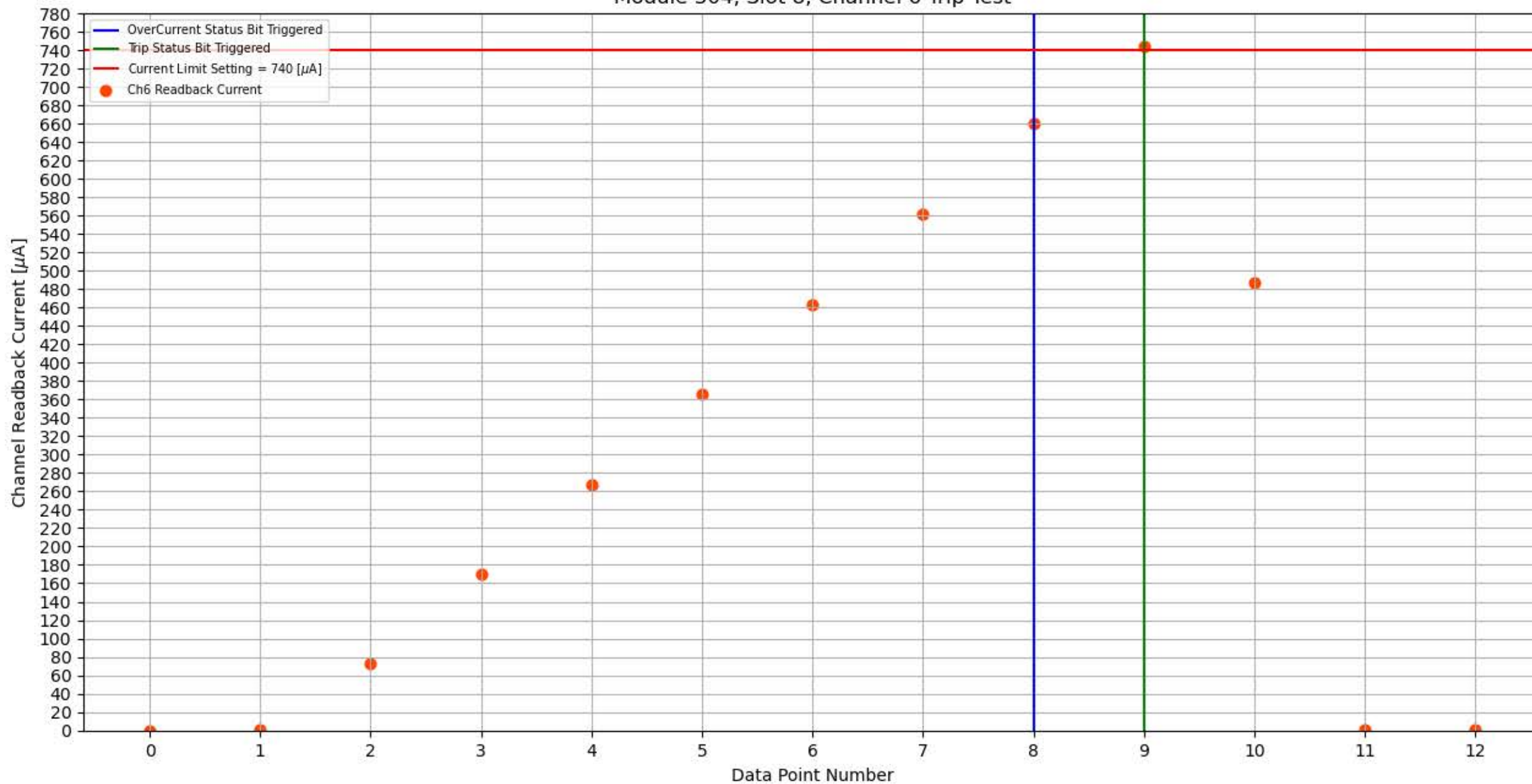
Module 304, Slot 8, Channel 6 Trip Test
