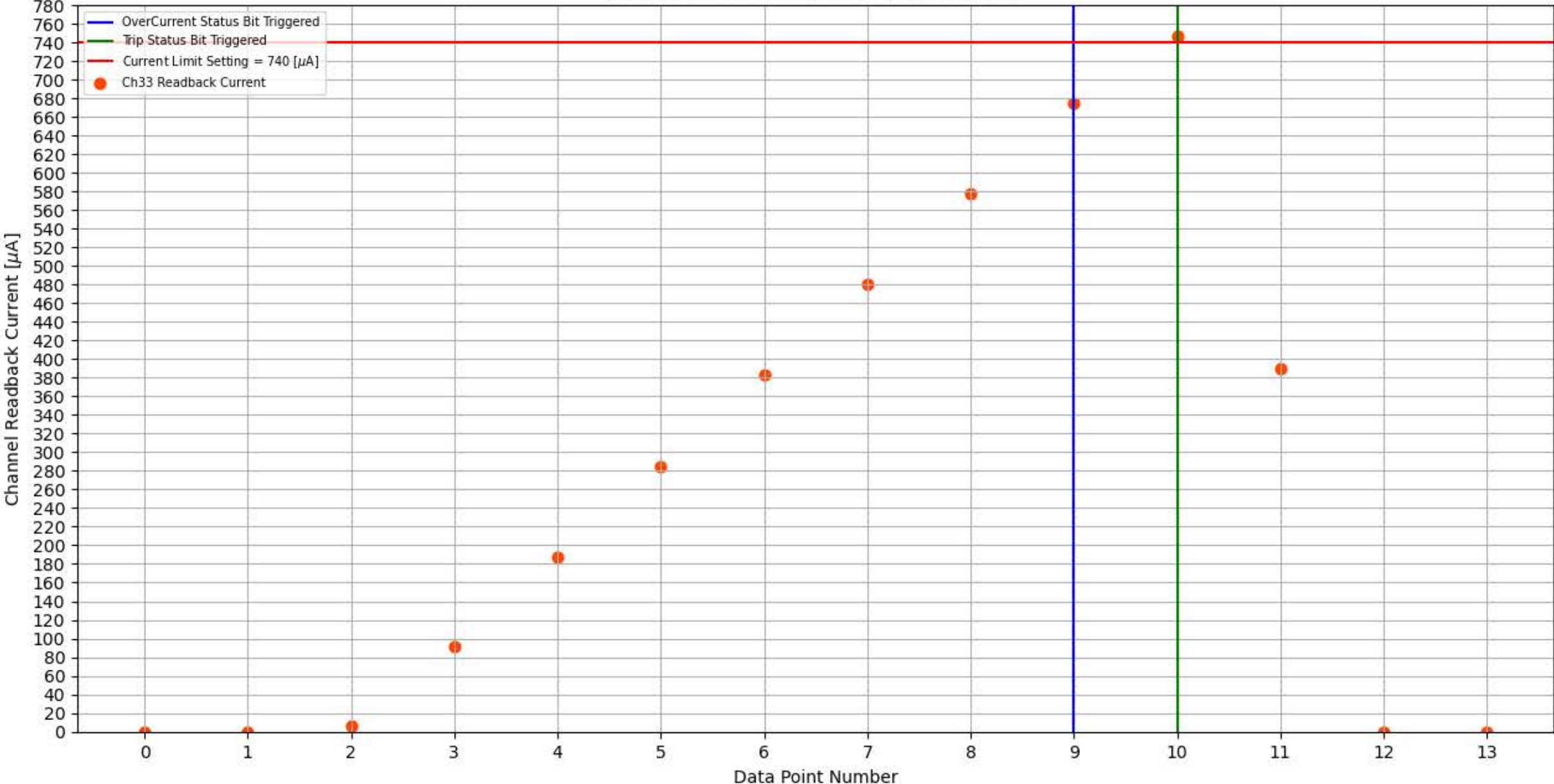
Module 304, Slot 8, Channel 33 Trip Test
