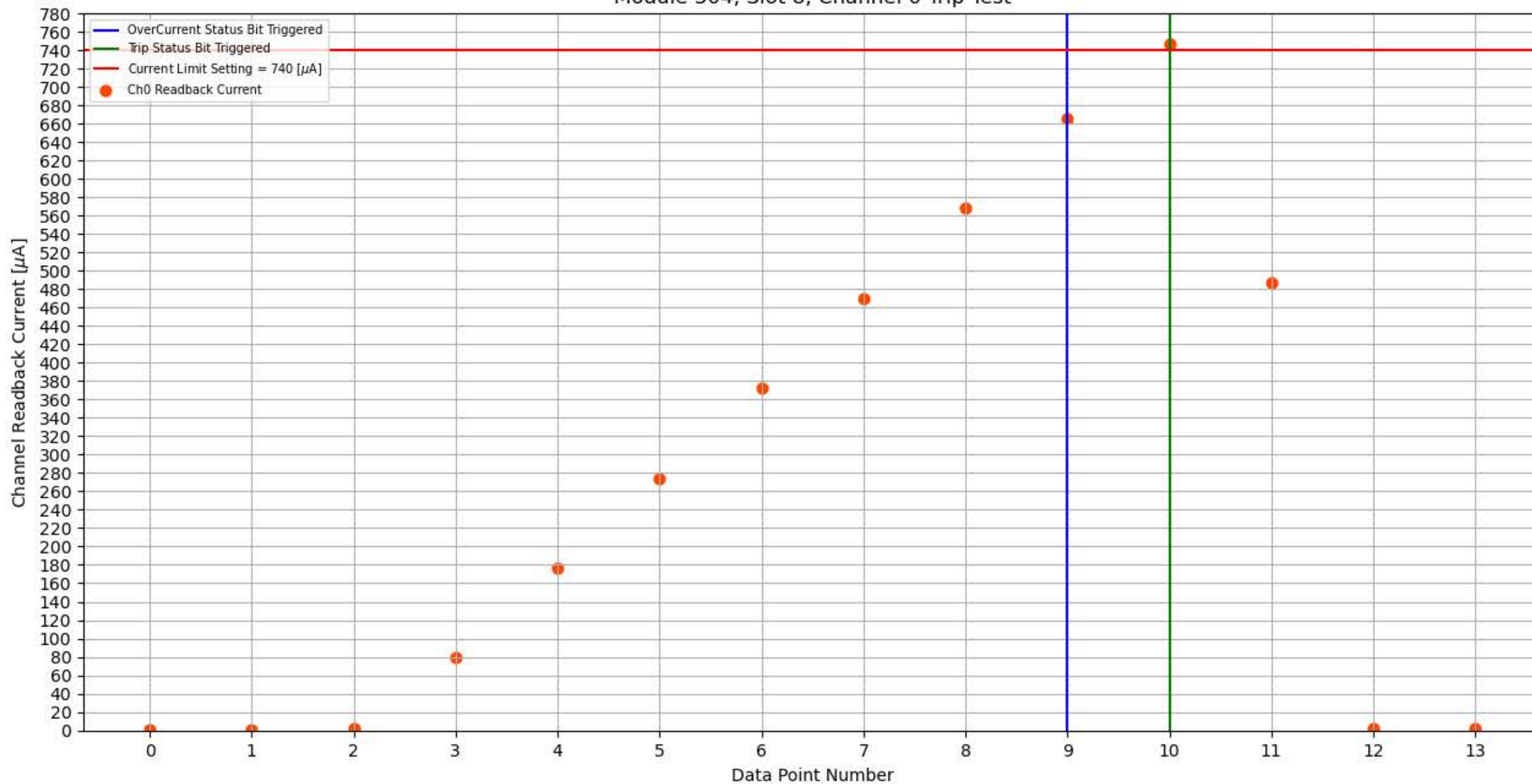
Module 304, Slot 8, Channel 0 Trip Test
