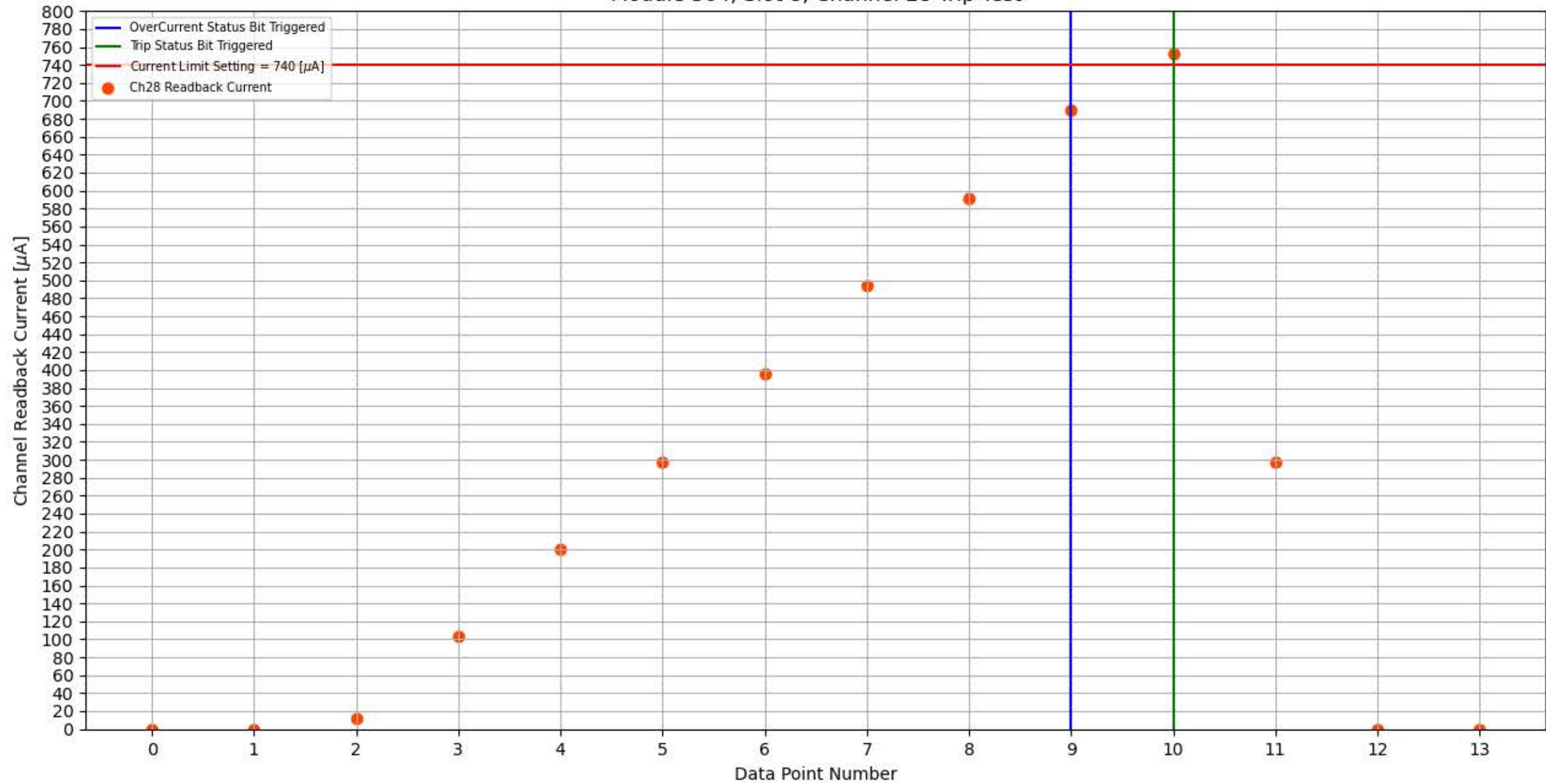
Module 304, Slot 8, Channel 28 Trip Test
