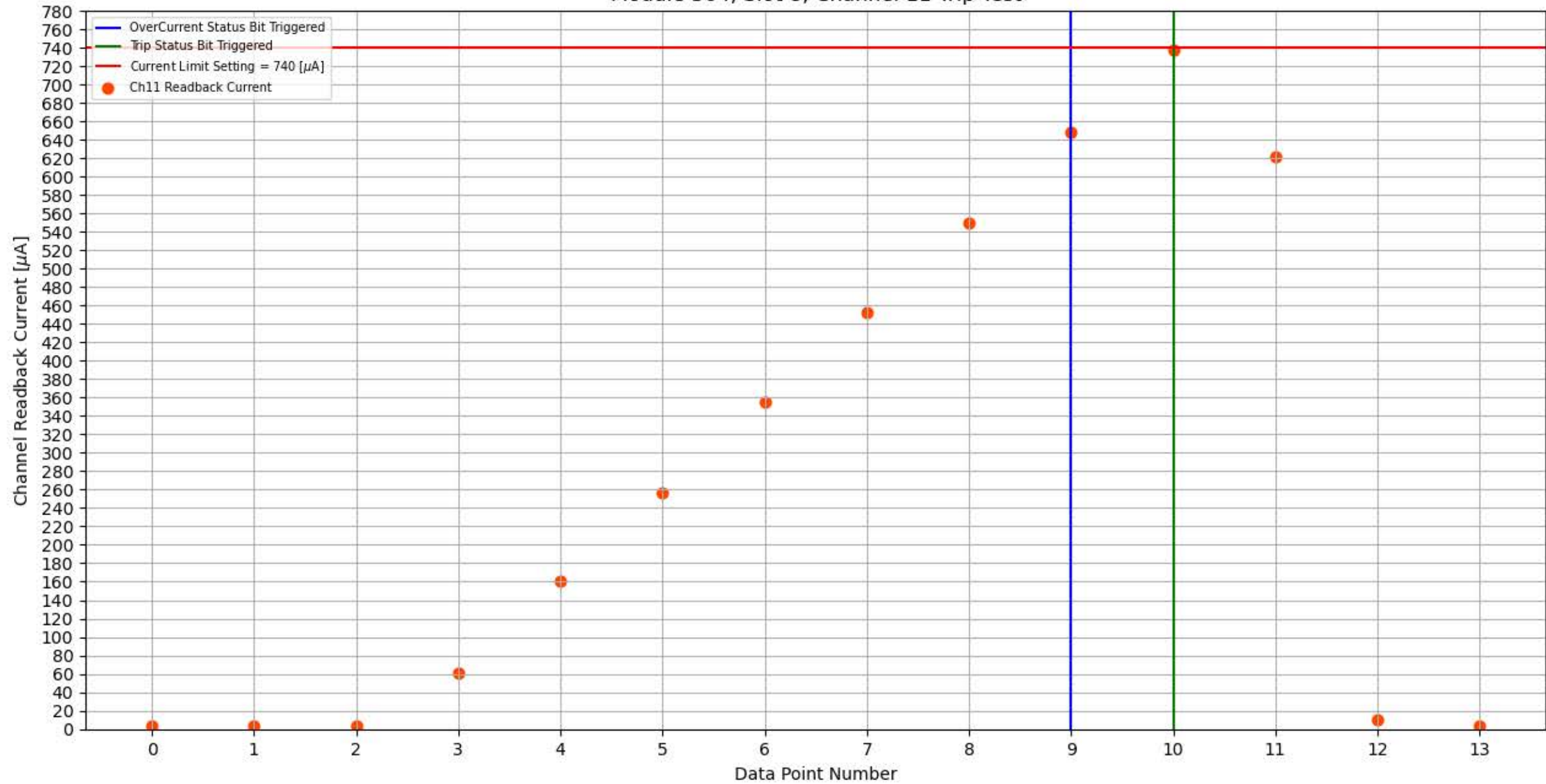
Module 304, Slot 8, Channel 11 Trip Test
