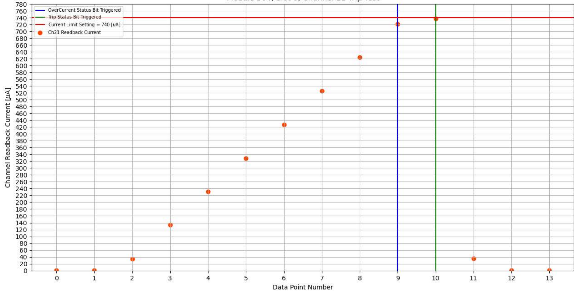
Module 304, Slot 8, Channel 21 Trip Test
