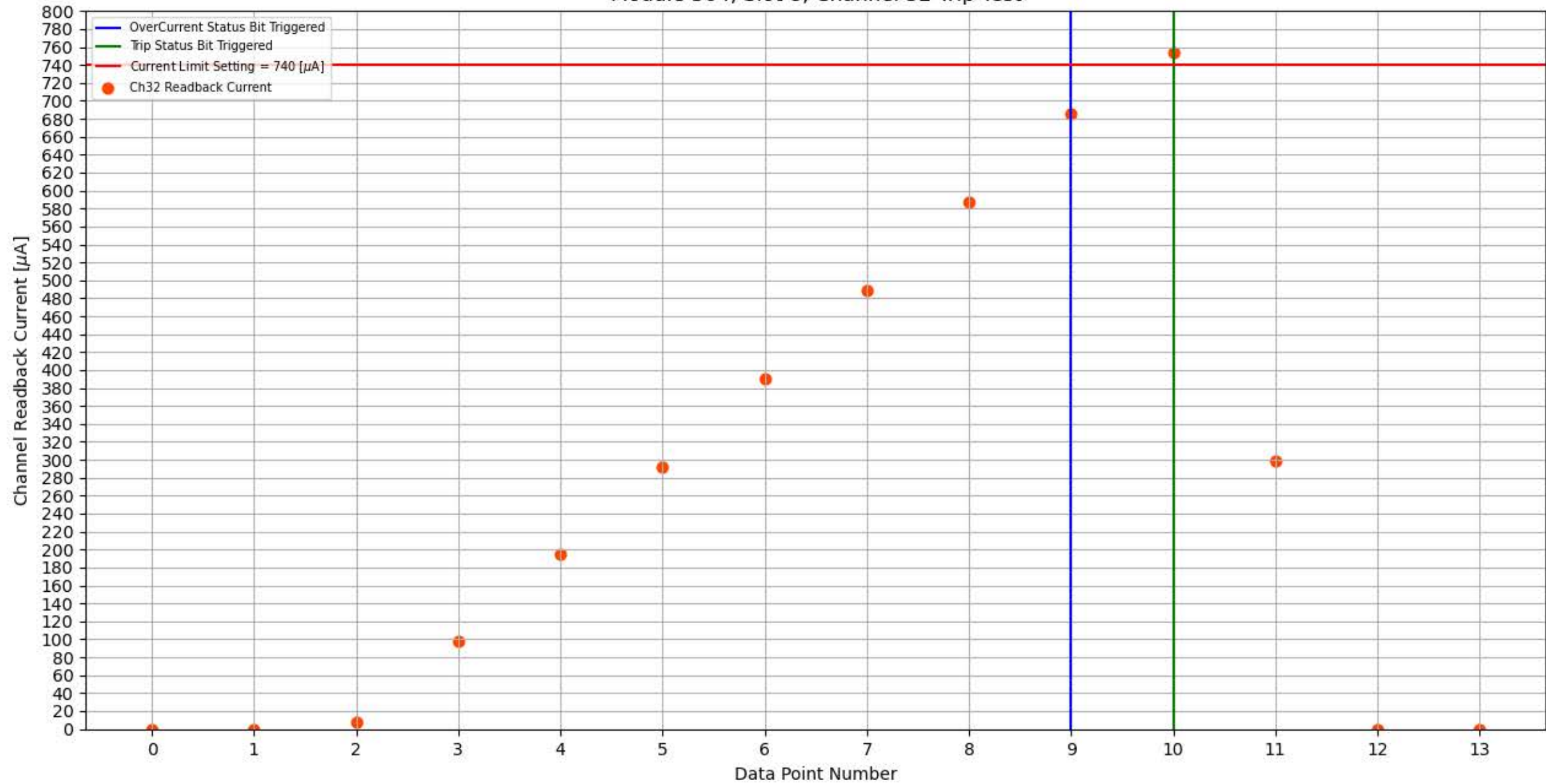
Module 304, Slot 8, Channel 32 Trip Test
