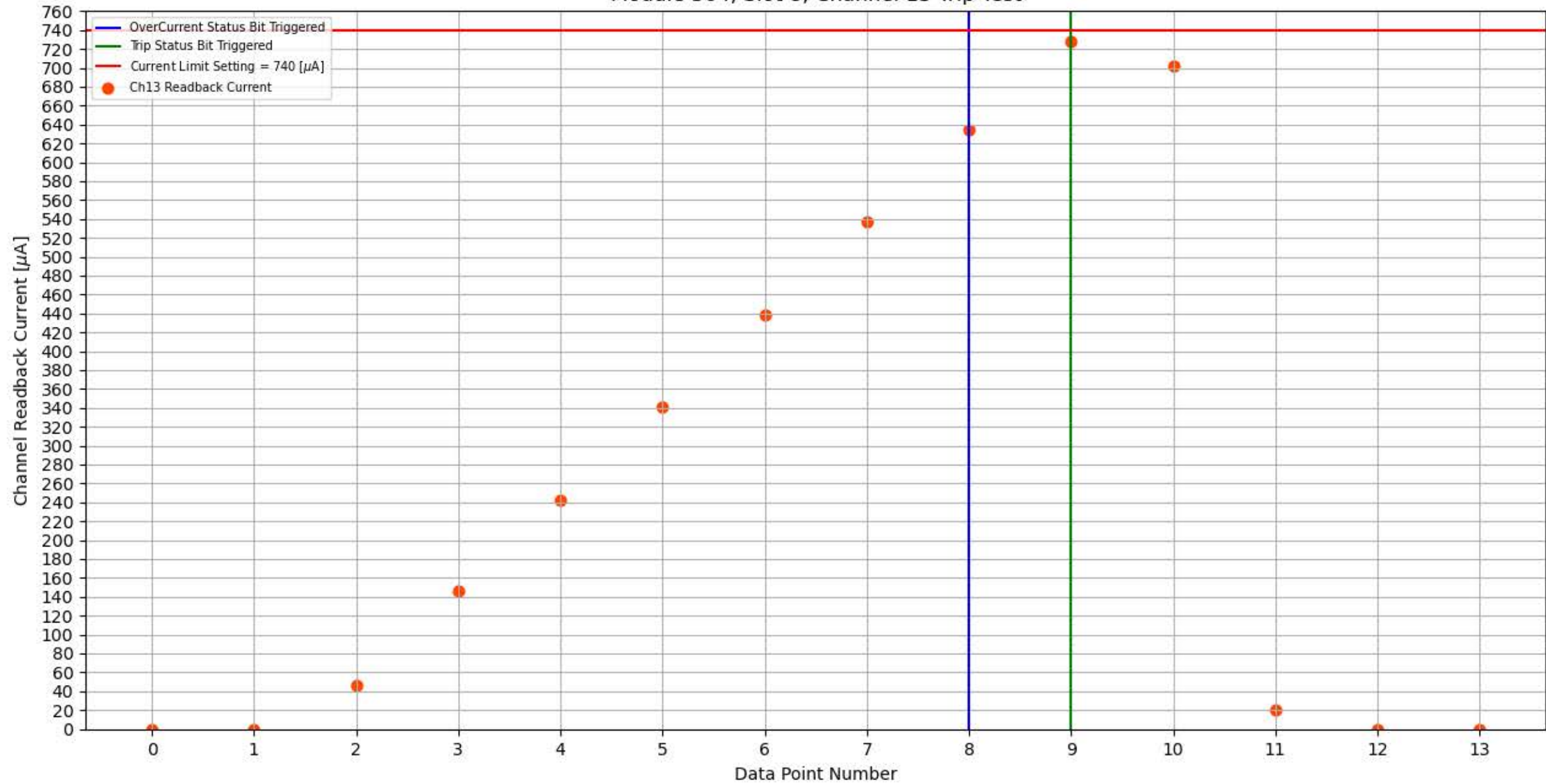
Module 304, Slot 8, Channel 13 Trip Test
