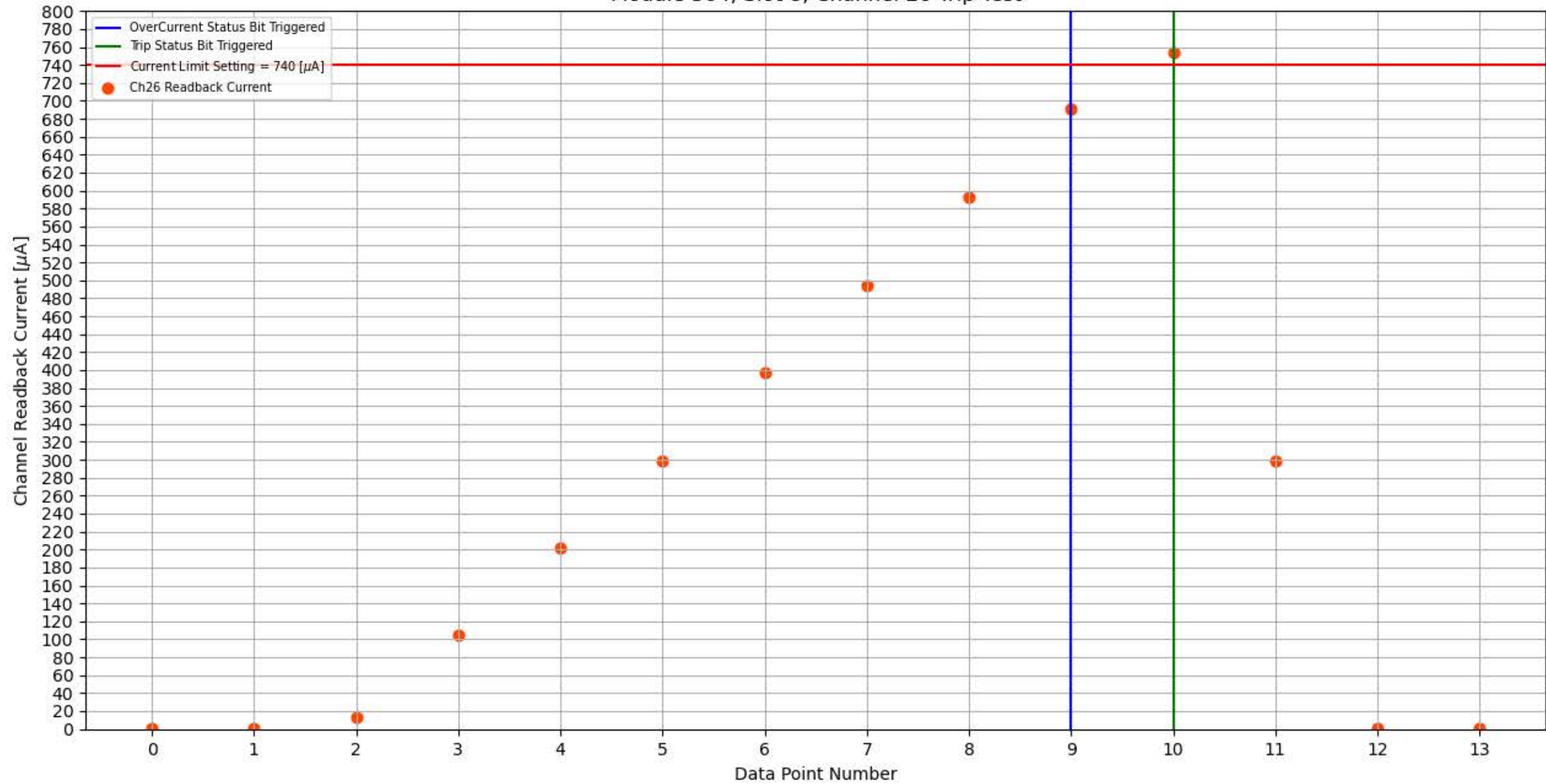
Module 304, Slot 8, Channel 26 Trip Test
